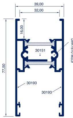
Ref. 4322 Hoja
