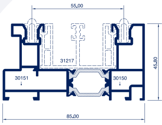
Ref. 4301 Marco
