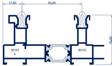
Ref. 4306 Marco
