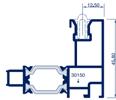
Ref. 4309 Marco
