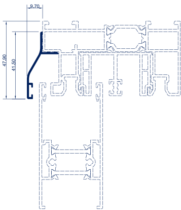
Ref. 4319 Goterón
