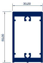
Ref. 3918
