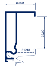
Ref. 4325 Cruce
