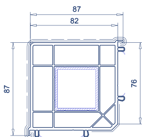
Ref. 116.229 Esquinera 90°, 87x87 mm Refuerzo 113.281.2
