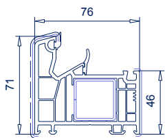
Ref. 101.350 Refuerzo 113.025 Marco SL76, 76 mm
