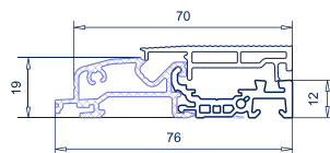
Ref. 104.530 Solera SL 76
