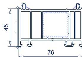
Ref. 114.054 Ensanche SL76, 45 mm
