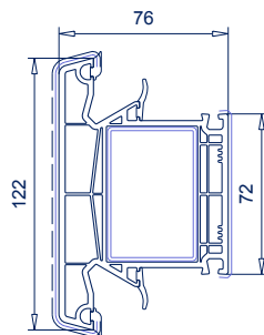
Ref. 102.351 113.011 Travesaño SL 76
