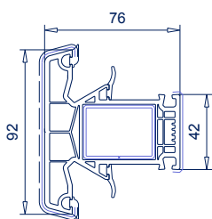
Ref. 102.350 113.001 & 113.367 Travesaño SL 76
