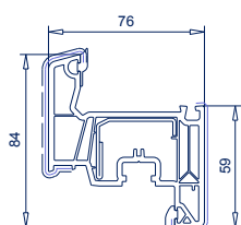
Ref. 103.381 113.292, 113.294, 113.295 & 113.394 Hoja SL76
