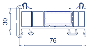
Ref. 114.053 Ensanche SL76, 30 mm Refuerzo 113.055
